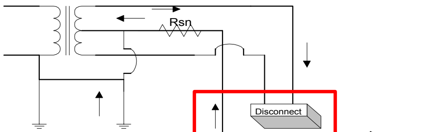
Figure 2 Neutral current flow on a three-wire service
