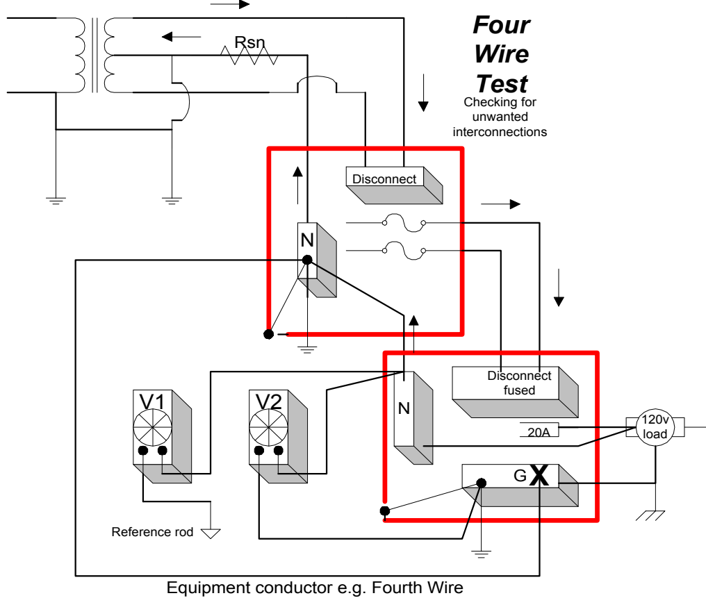
Figure 4 Setup for testing four-wire systems
