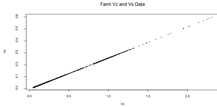
Figure 4. Vs and Vcr Data from the Waverider data acquisition System.
