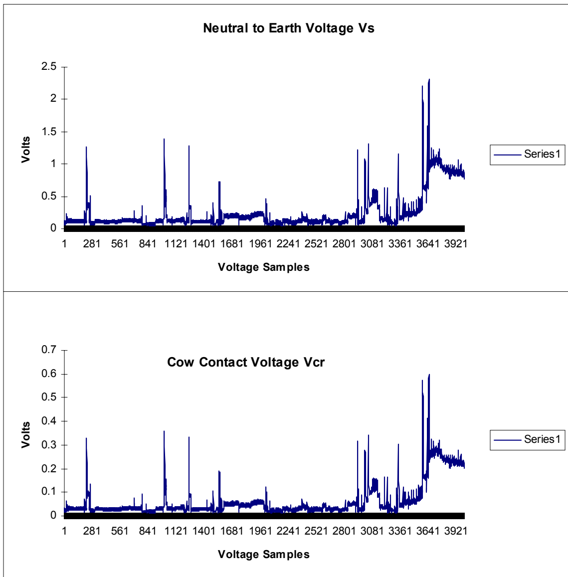
Figure 4. Vs and Vcr Data from the Waverider data acquisition System.
