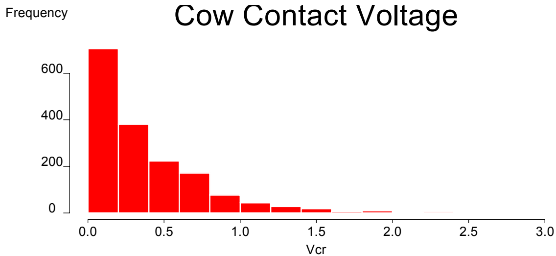
Figure 2. Cow Contact Voltages (Vcr) on 1700 Wisconsin Farms.
